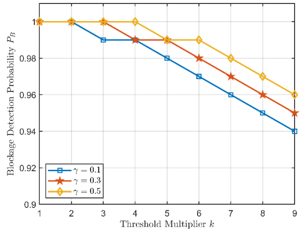
Fig 3: Blockage Detection Probability versus Threshold Multiplier
