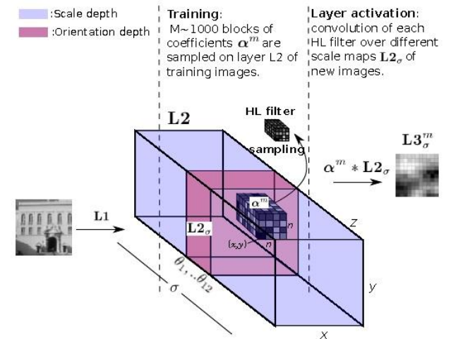
Fig. 4 Third level of HMAX: in training Phase, M \sim 1000 HL filters is defined by L2 coefficients of sampling blocks. Layer activation in each image is obtained by convolving each HL filter on all positions of each L2_{\sigma} scale map [5].
