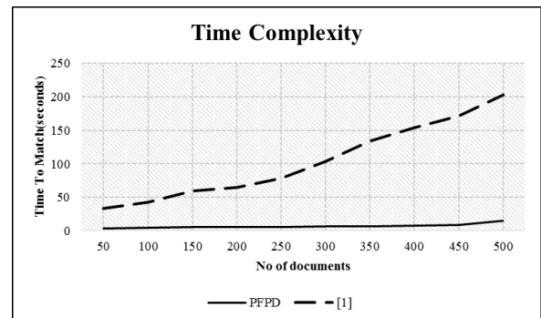
Fig. 8. Time Complexity
